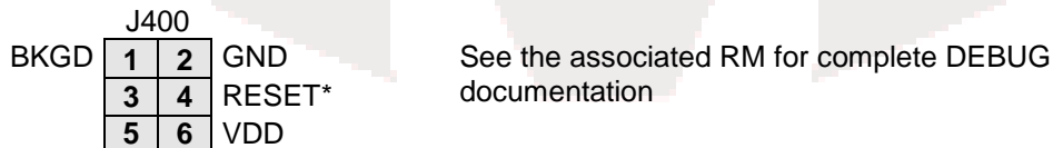
Figure 2: BDM_PORT Header
