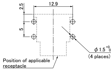
HR12-10R-SP(71) (Stopper Plate) (Applicable PCB thickness: 1 to 2mm)
