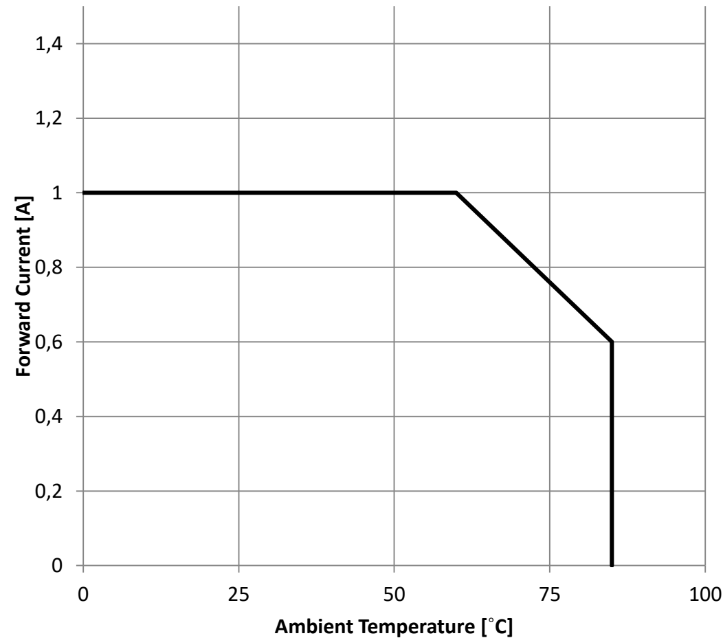
Derating Curve:
