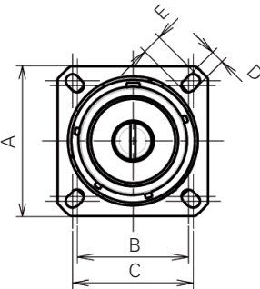
8D0 Square flange receptacle
