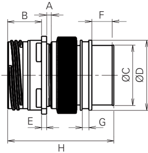
With 8D0 (square flange receptacle)
