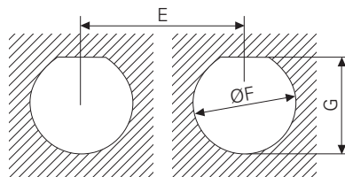
Jam nut receptacle (Type 7)
