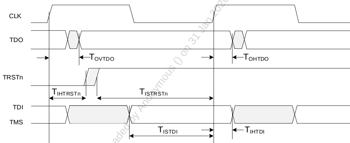
Figure 17. JTAG Timing
