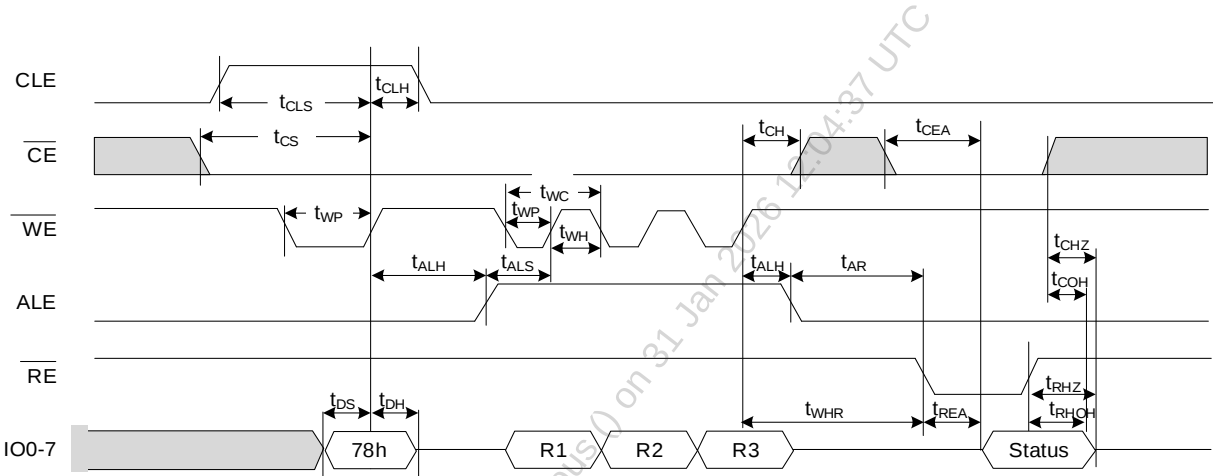
Figure 29. Read Status Enhanced Timing
