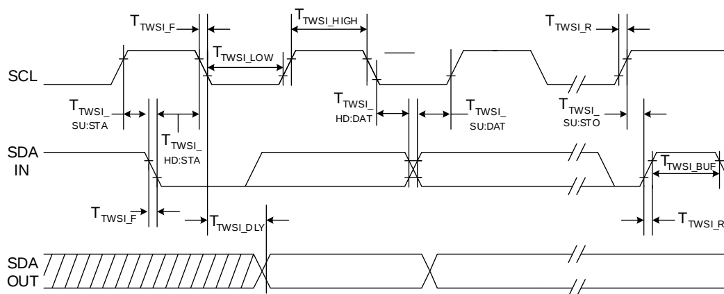
Figure 13. Two-wire serial interface timing
