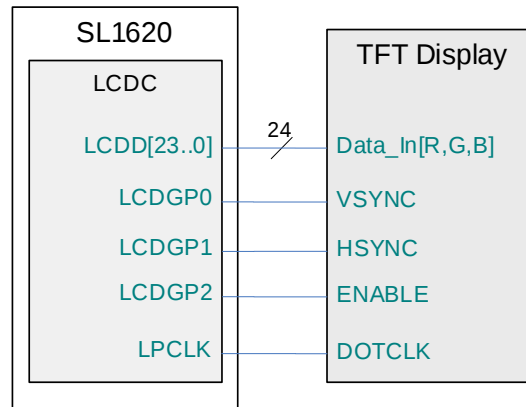
Figure 33. LCDDC TFT Interface Connectivity
