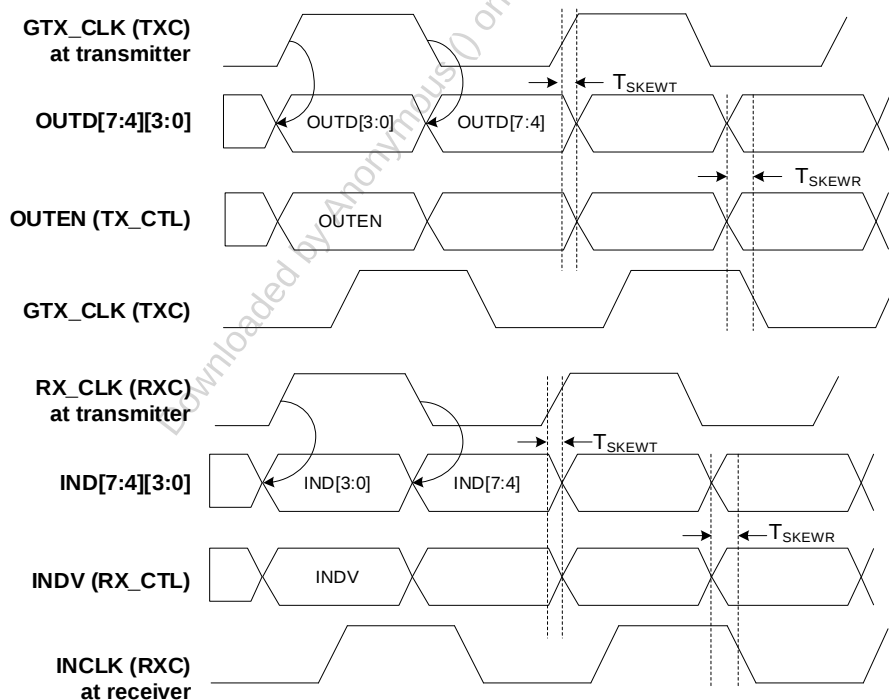
Figure 16. RGMII Timing
