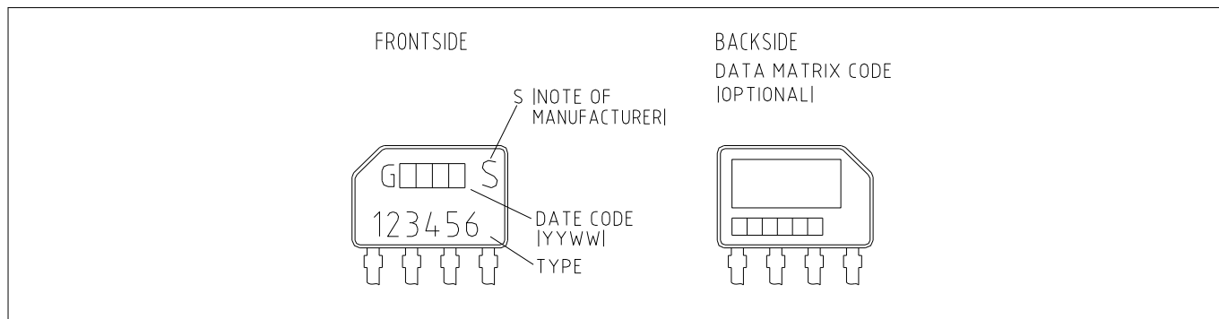
Figure 9 Marking pattern
