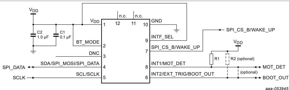
Figure 27. Typical Application Circuit #6 - Motion detection mode (with SPI 3-wire interface, software enabled)
