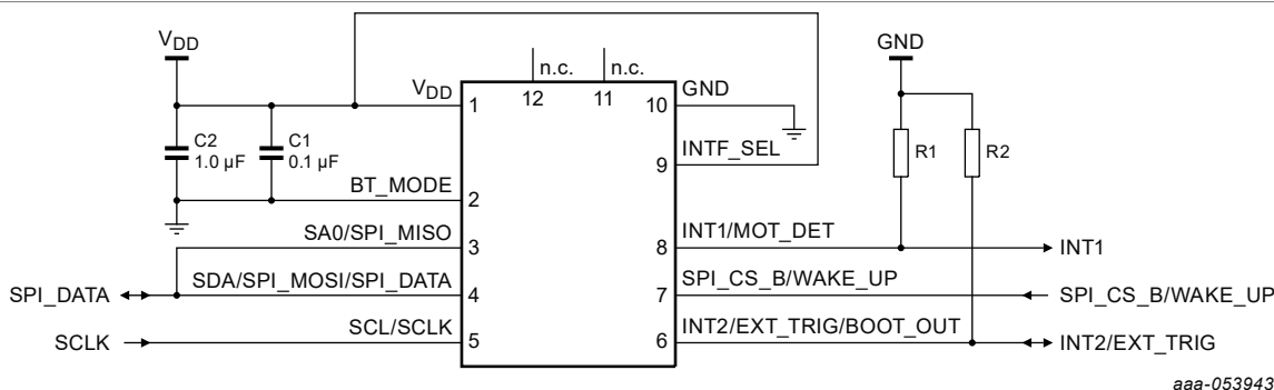
Figure 25. Typical Application Circuit #4 – SPI 3-wire mode (hardwired; SENS_CONFIG1[SPI_M] = X)
