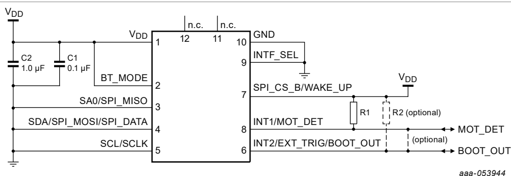
Figure 26. Typical Application Circuit #5 – Motion detection mode (no serial interface)
