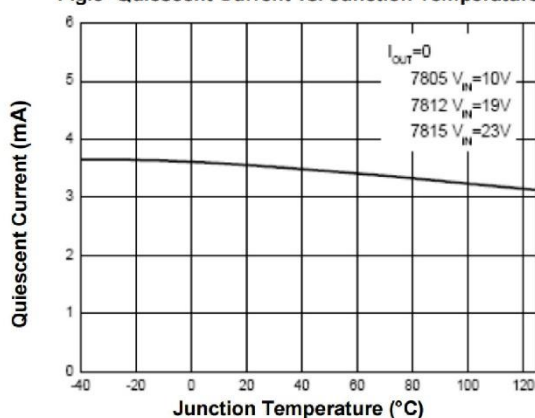
Fig.3- Quiescent Current vs. Junction Temperature
