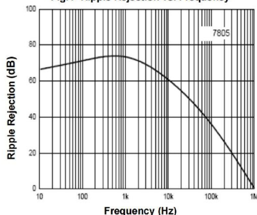
Fig.4- Ripple Rejection vs. Frequency
