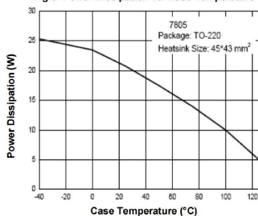
Fig.6- Power Dissipation vs. Case Temperature
