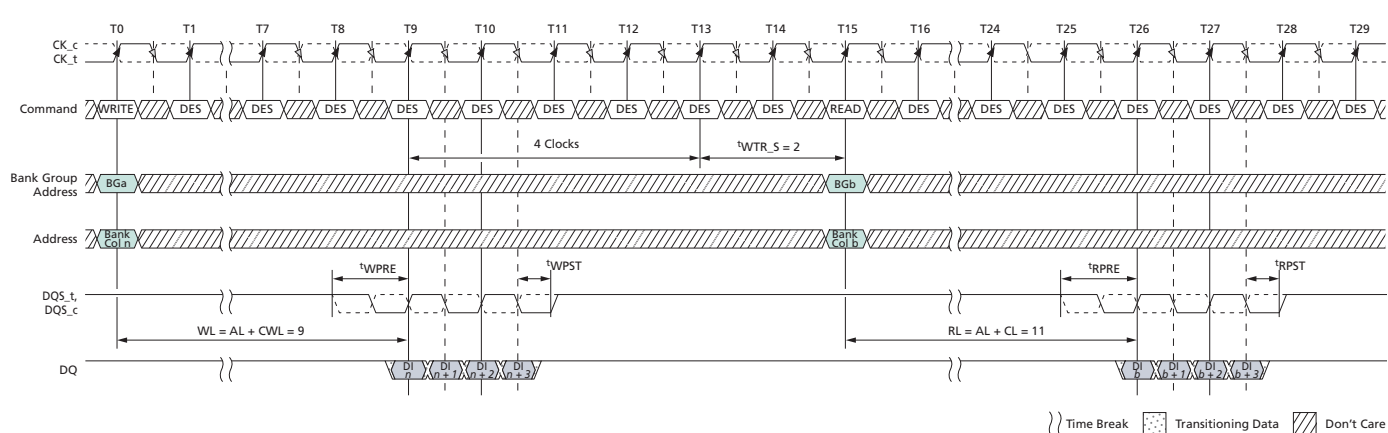
Figure 185: WRITE (BC4) OTF to READ (BC4) OTF with 1^{\text{t}} CK Preamble in Different Bank Group
