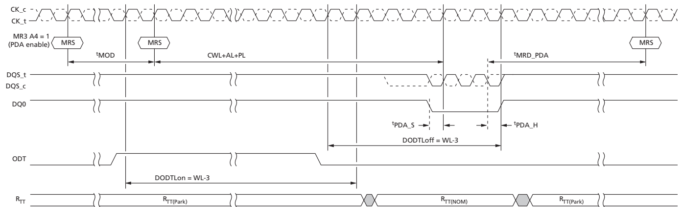
Figure 62: PDA Operation Enabled, BC4
