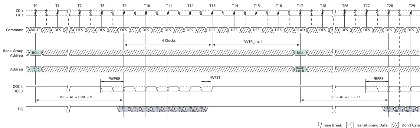
Figure 184: WRITE (BL8) to READ (BL8) with 1^{\text{t}} CK Preamble in Same Bank Group
