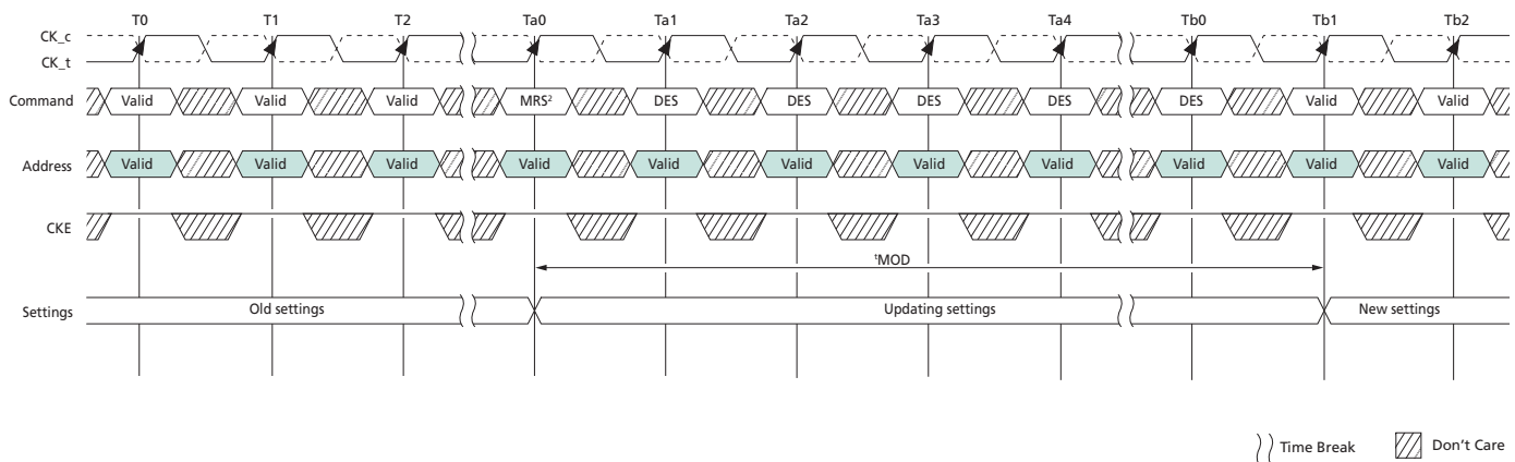
Figure 17: t_{MOD} Timing
