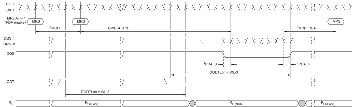
Figure 61: PDA Operation Enabled, BL8
