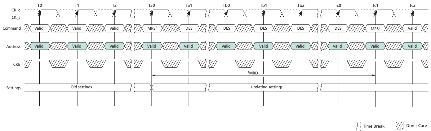
Figure 16: t_{MRD} Timing
