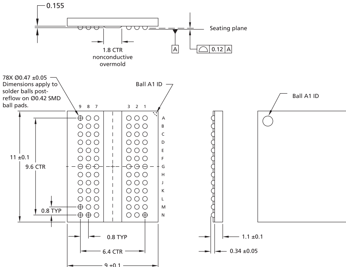
Figure 8: 78-Ball FBGA – x4, x8 (JC)
