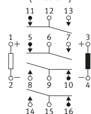
2 coil latching ( Reset )
