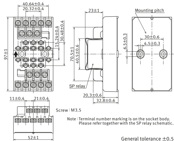
External dimensions
