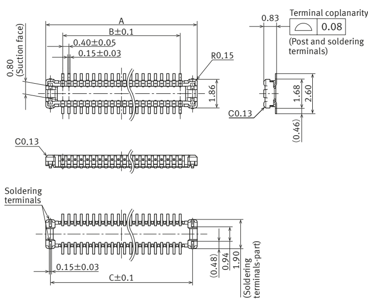
External dimensions
