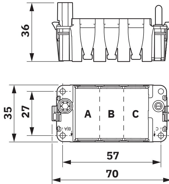
Dimensional drawing
