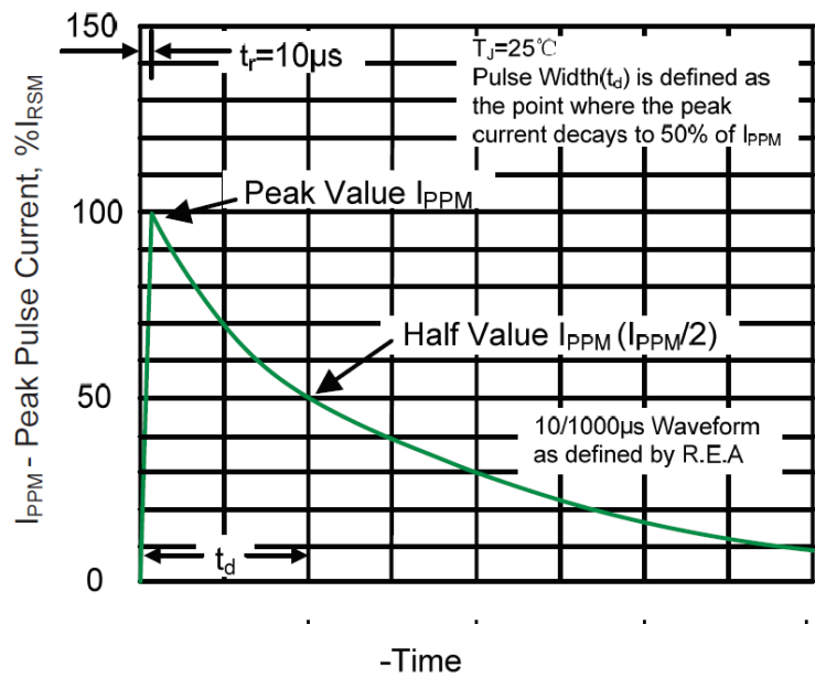
Figure 3. Pulse Waveform
