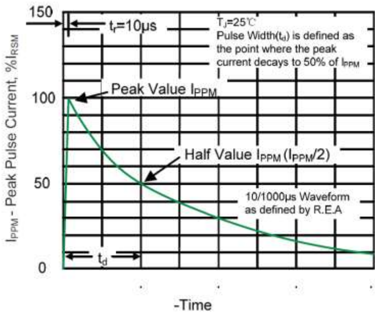
Figure 3. Pulse Waveform
