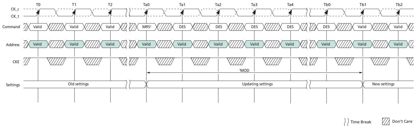
Figure 17: t^{\text{MOD}} Timing
