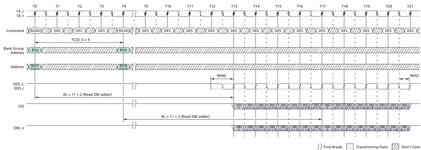
Figure 156: Consecutive READ (BL8) with 1 st CK Preamble and DBI in Different Bank Group
