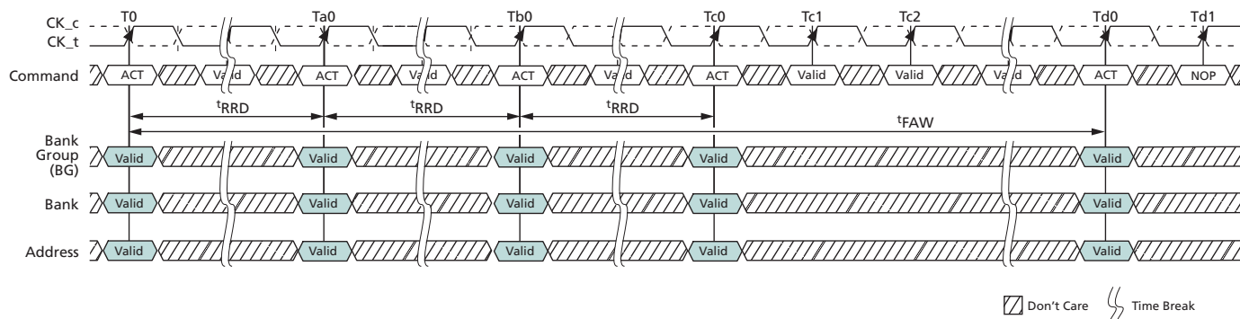
Figure 81: t_{FAW} Timing
