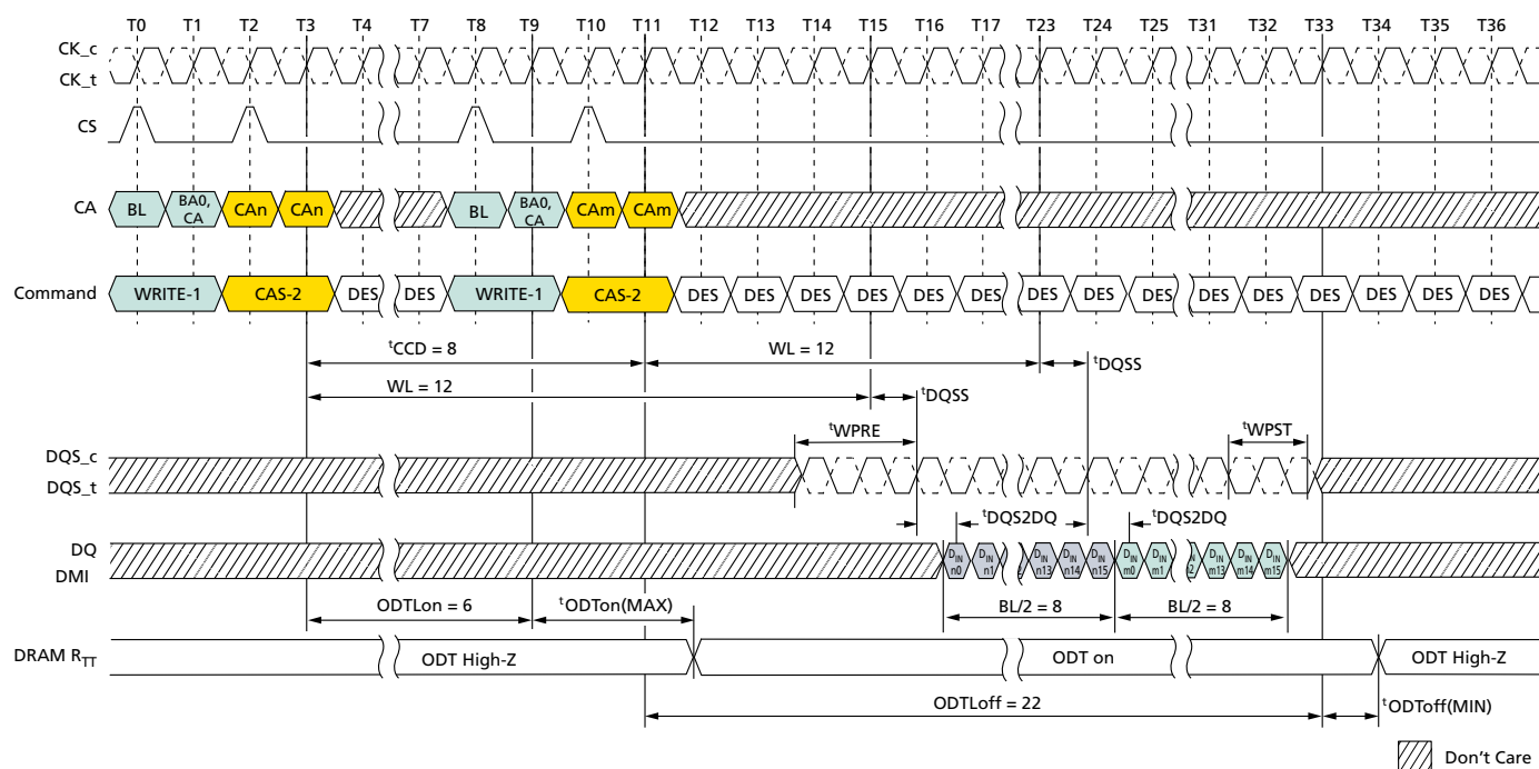
Figure 57: Seamless WRITE: t_{\text{CCD}} = \text{MIN} , 1.5n\text{CK} Postamble, 533 \text{ MHz} < \text{Clock Frequency} \leq 800 \text{ MHz} , ODT Worst Timing Case
