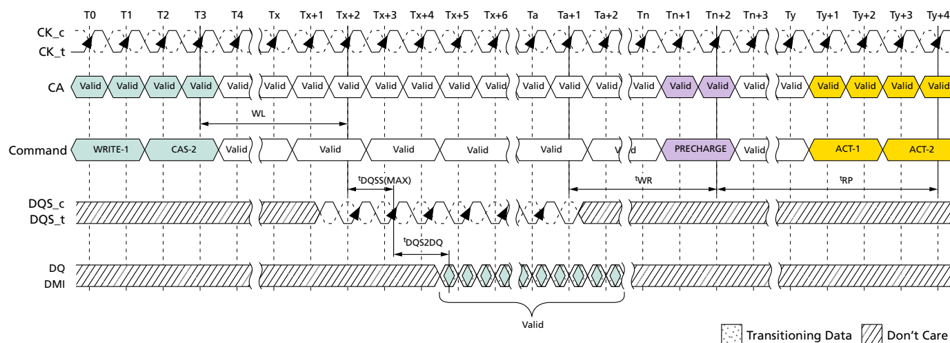
Figure 68: Burst WRITE Followed by PRECHARGE – BL16, 2nCK Preamble, 0.5nCK Postamble
