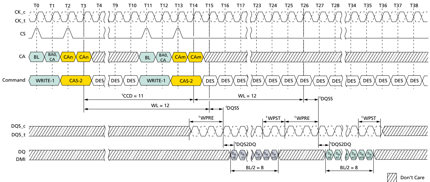
Figure 64: Consecutive WRITE: t_{CCD} = \text{MIN} + 3, 1.5nCK Postamble
