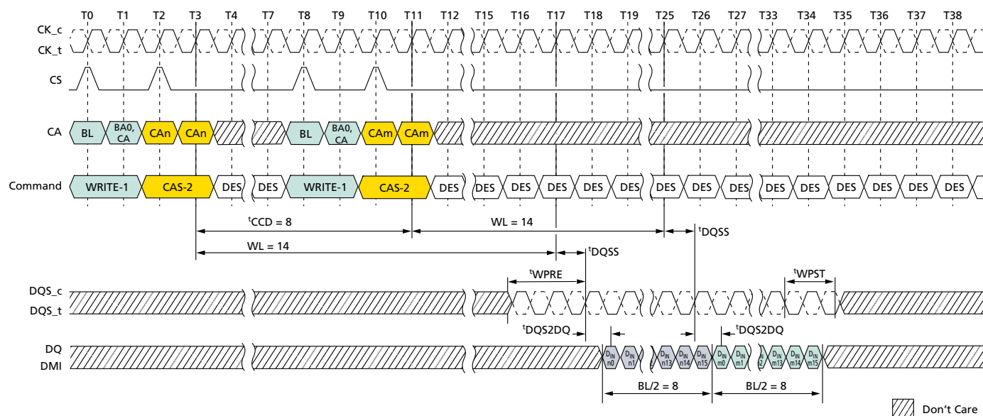
Figure 58: Seamless WRITE: t_{\text{CCD}} = \text{MIN} , 1.5n\text{CK} Postamble
