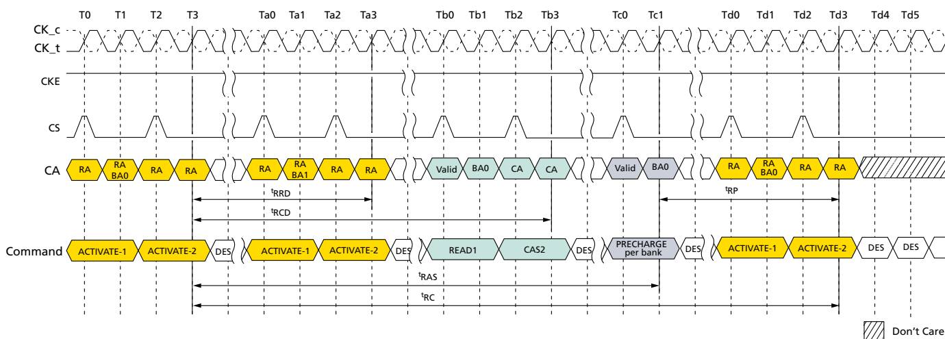
Figure 16: ACTIVATE Command
