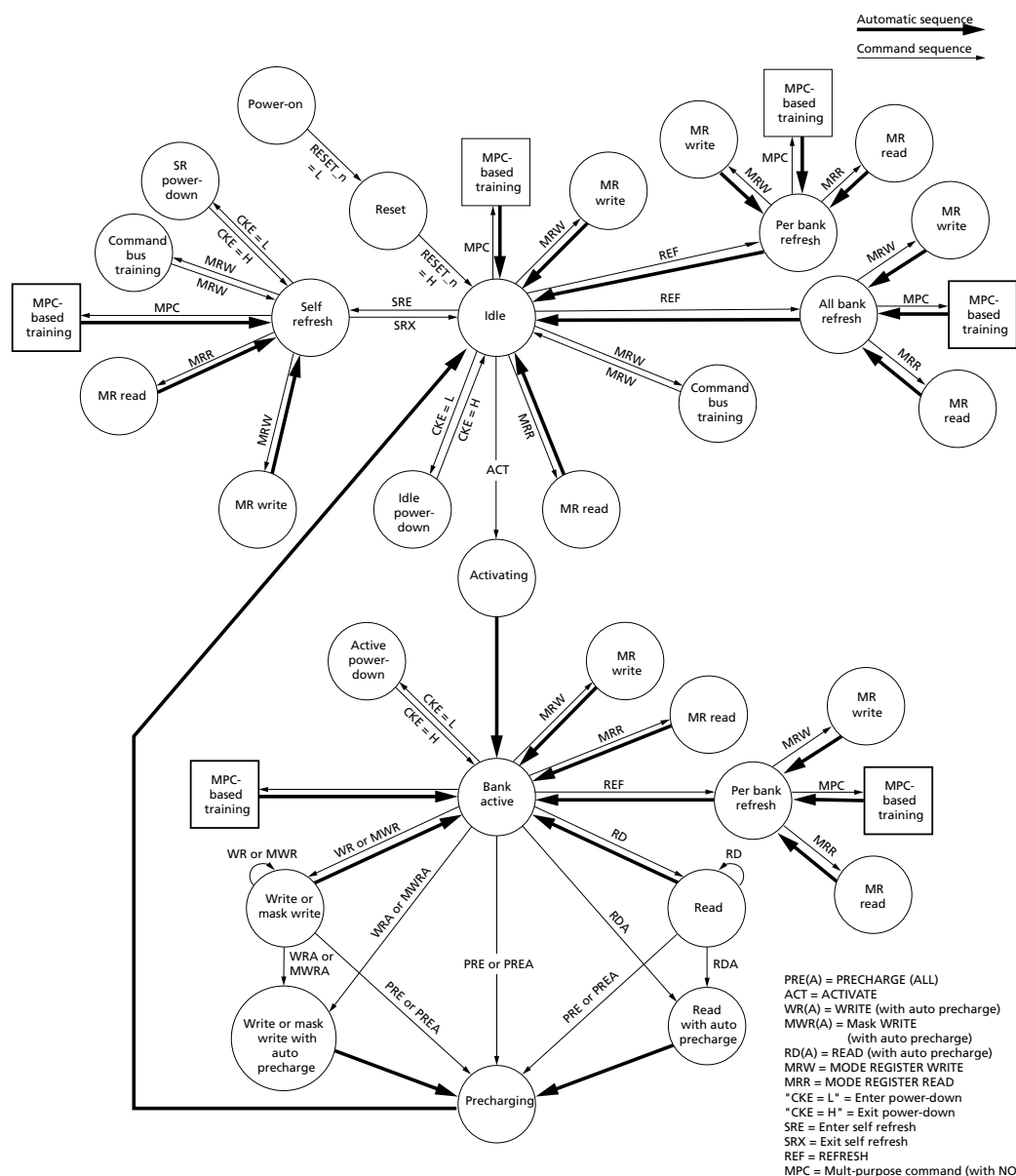
Figure 13: Simplified State Diagram
