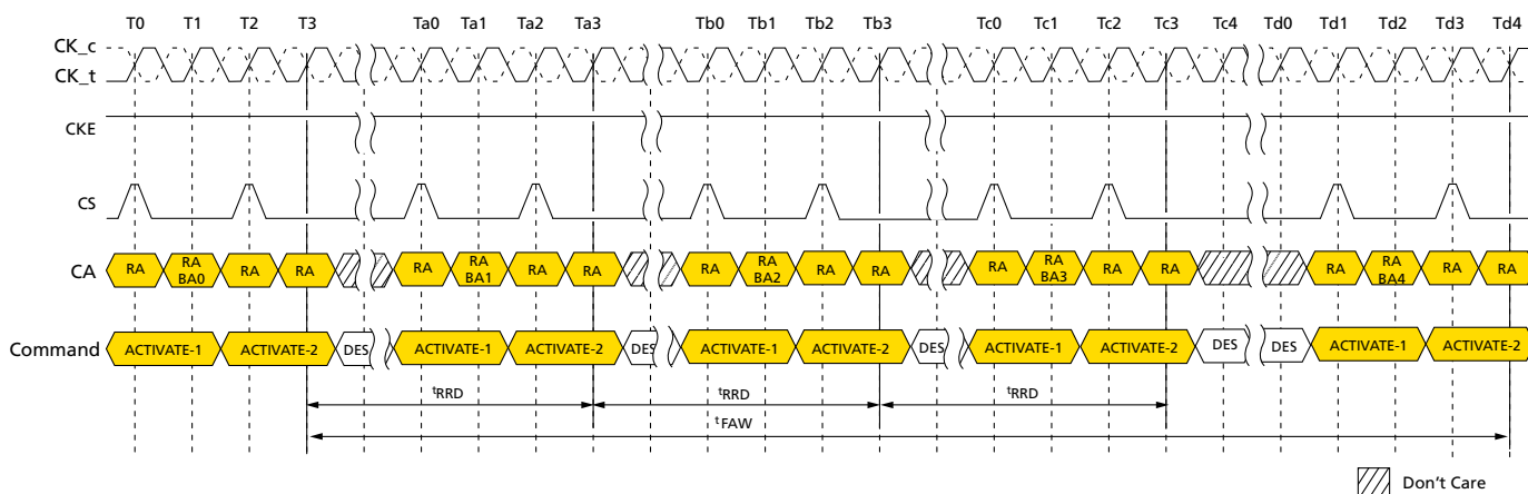
Figure 17: t_{FAW} Timing
