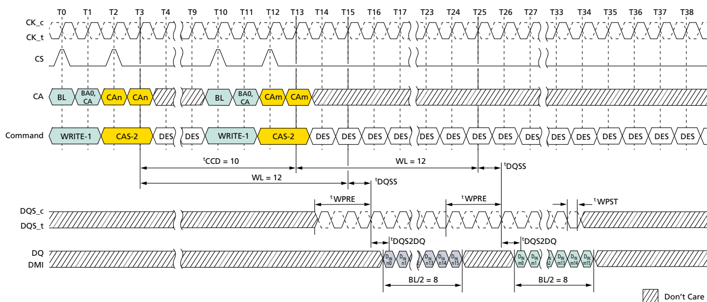
Figure 61: Consecutive WRITE: t_{CCD} = \text{MIN} + 2, 0.5n\text{CK} Postamble
