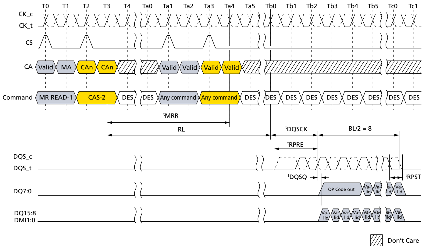
Figure 95: MODE REGISTER READ Operation
