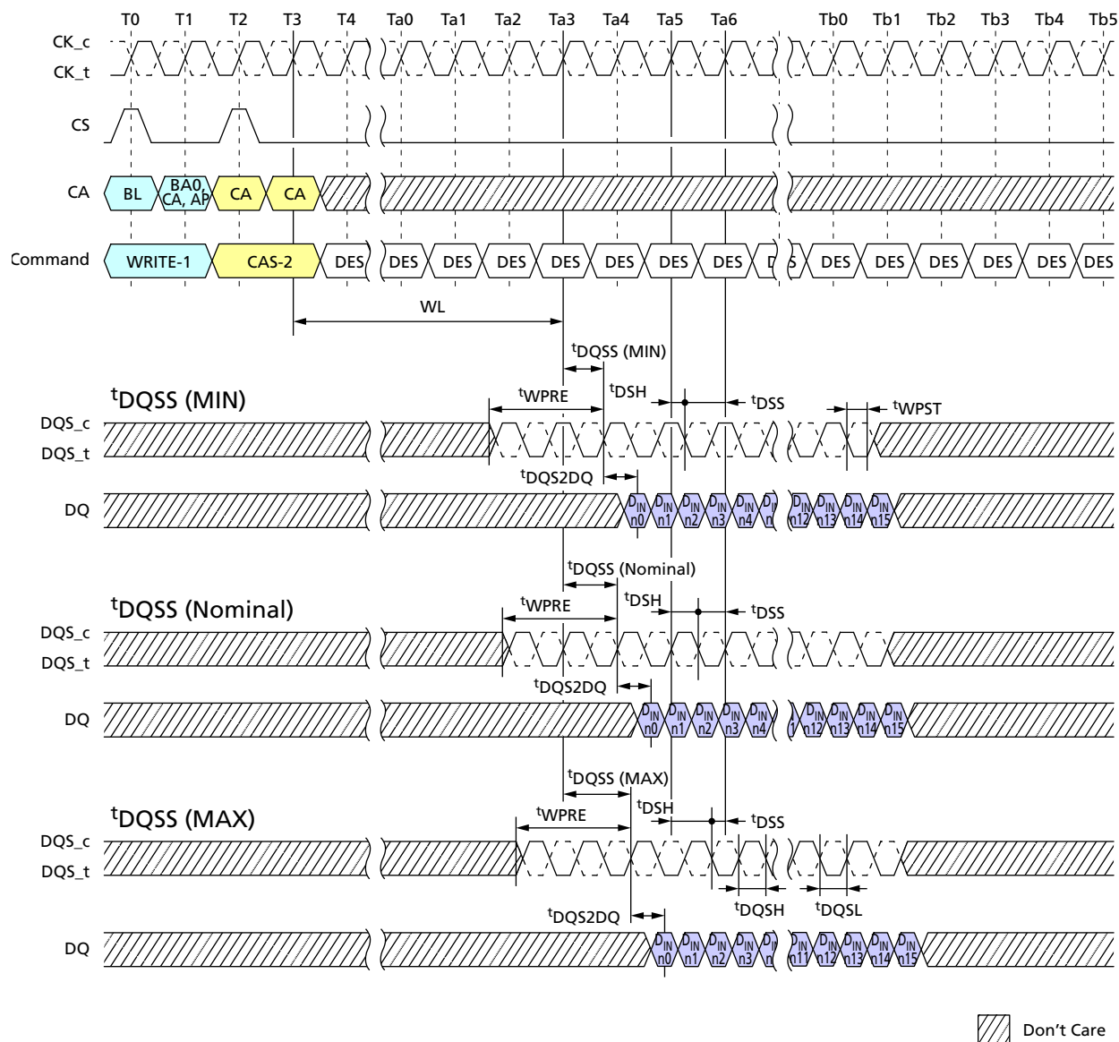
Figure 32: Write Timing
