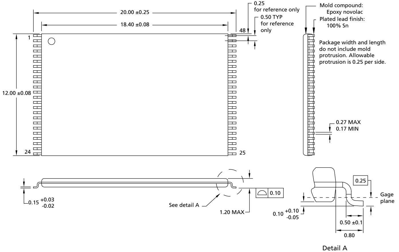
Figure 4: 48-Pin TSOP – Type 1 CPL (Package Code: WP)
