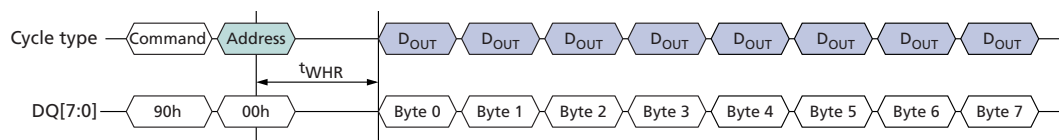
Figure 30: READ ID (90h) with 00h Address Operation
