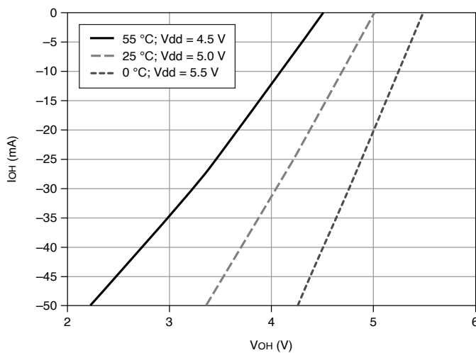
Figure 2. P0.<0..31>: I_{OH} versus V_{OH}
