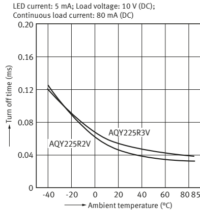
4-2. Turn off time vs. ambient temperature characteristics
