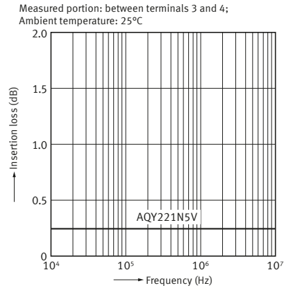
15-2. Insertion loss vs. frequency characteristics ( 50 Ω impedance )
