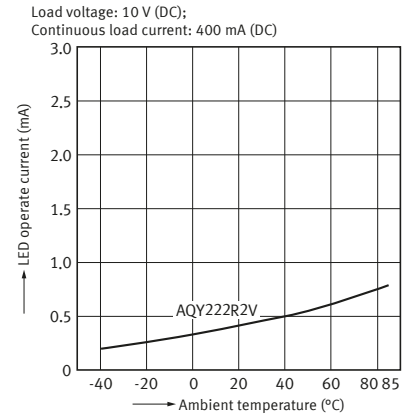
5-1. LED operate current vs. ambient temperature characteristics
