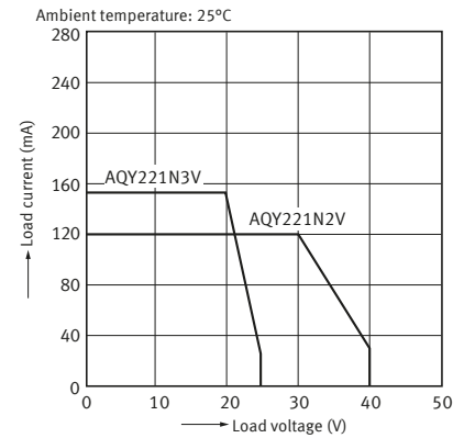
2-1. Load current vs. load voltage characteristics
