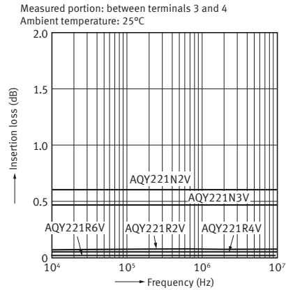
15-1. Insertion loss vs. frequency characteristics ( 50 Ω impedance )
