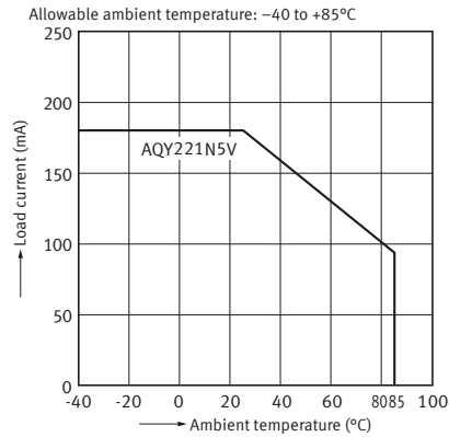
1-2. Load current vs. ambient temperature characteristics
