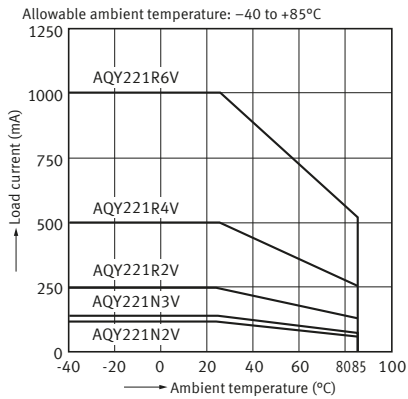
1-1. Load current vs. ambient temperature characteristics
