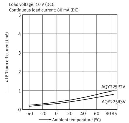
6-2. LED turn off current vs. ambient temperature characteristics
