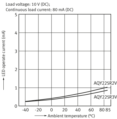
5-2. LED operate current vs. ambient temperature characteristics
