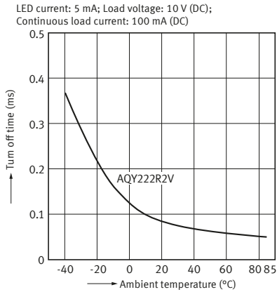
4-1. Turn off time vs. ambient temperature characteristics
