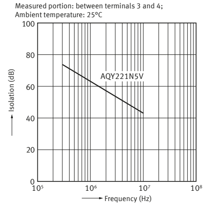
14-2. Isolation vs. frequency characteristics ( 50 Ω impedance )
