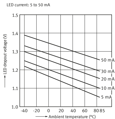
7. LED dropout voltage vs. ambient temperature characteristics
