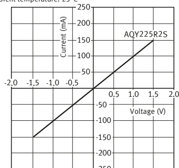
8-3. Current vs. voltage characteristics of output at MOS portion
