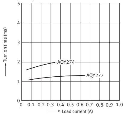
13-2. Turn on time vs. load current characteristics
