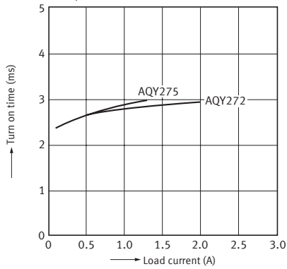
13-1. Turn on time vs. load current characteristics
