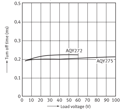
14-1. Turn off time vs. load voltage characteristics
