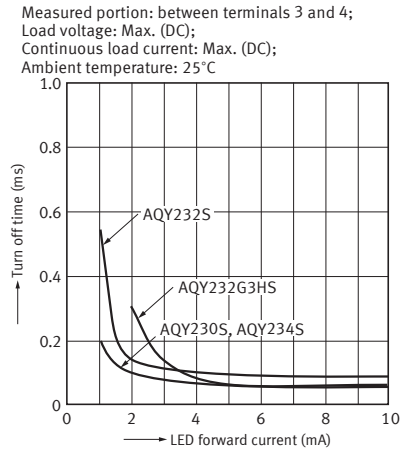
12. Turn off time vs. LED forward current characteristics
