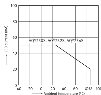
2-1. LED current vs. ambient temperature characteristics
