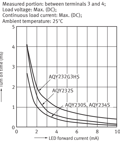
11. Turn on time vs. LED forward current characteristics
