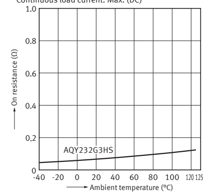
3-2. On resistance vs. ambient temperature characteristics
