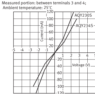
9-2. Current vs. voltage characteristics of output at MOS portion
