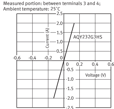
9-3. Current vs. voltage characteristics of output at MOS portion
