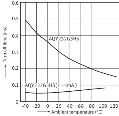
5-2. Turn off time vs. ambient temperature characteristics
