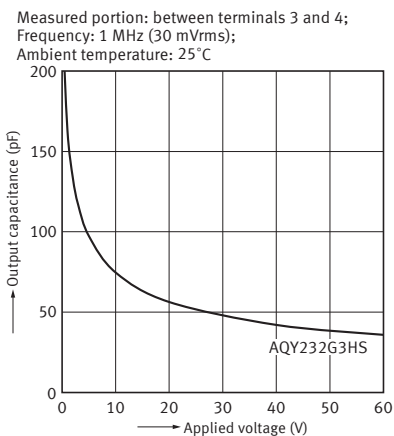
13-2. Output capacitance vs. applied voltage characteristics
