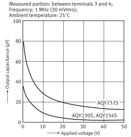
13-1. Output capacitance vs. applied voltage characteristics
