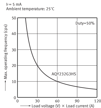
14. Max. operating frequency vs. load voltage and load current characteristics
