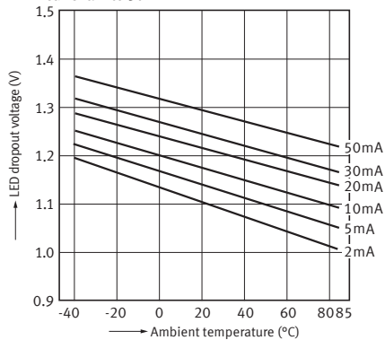
8-1. LED dropout voltage vs. ambient temperature characteristics
