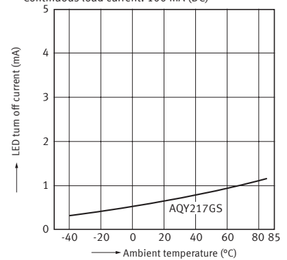
6-2. LED turn off current vs. ambient temperature characteristics
