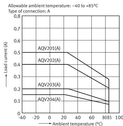
1-2. Load current vs. ambient temperature characteristics ( AC/DC type )
