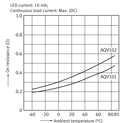
2-1. On resistance vs. ambient temperature characteristics ( DC type: AQV101, AQV102 )
