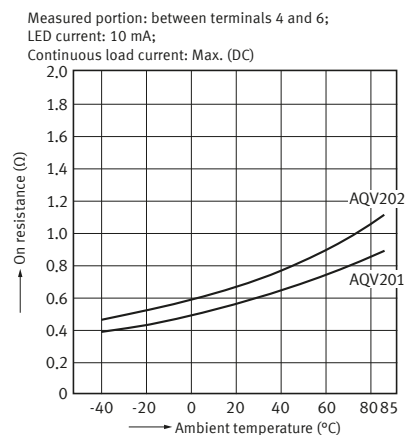
2-3. On resistance vs. ambient temperature characteristics ( AC/DC type: AQV201, AQV202 )
