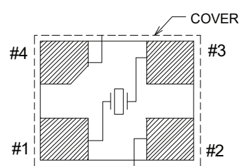
PIN CONNECTION (TOP VIEW)
