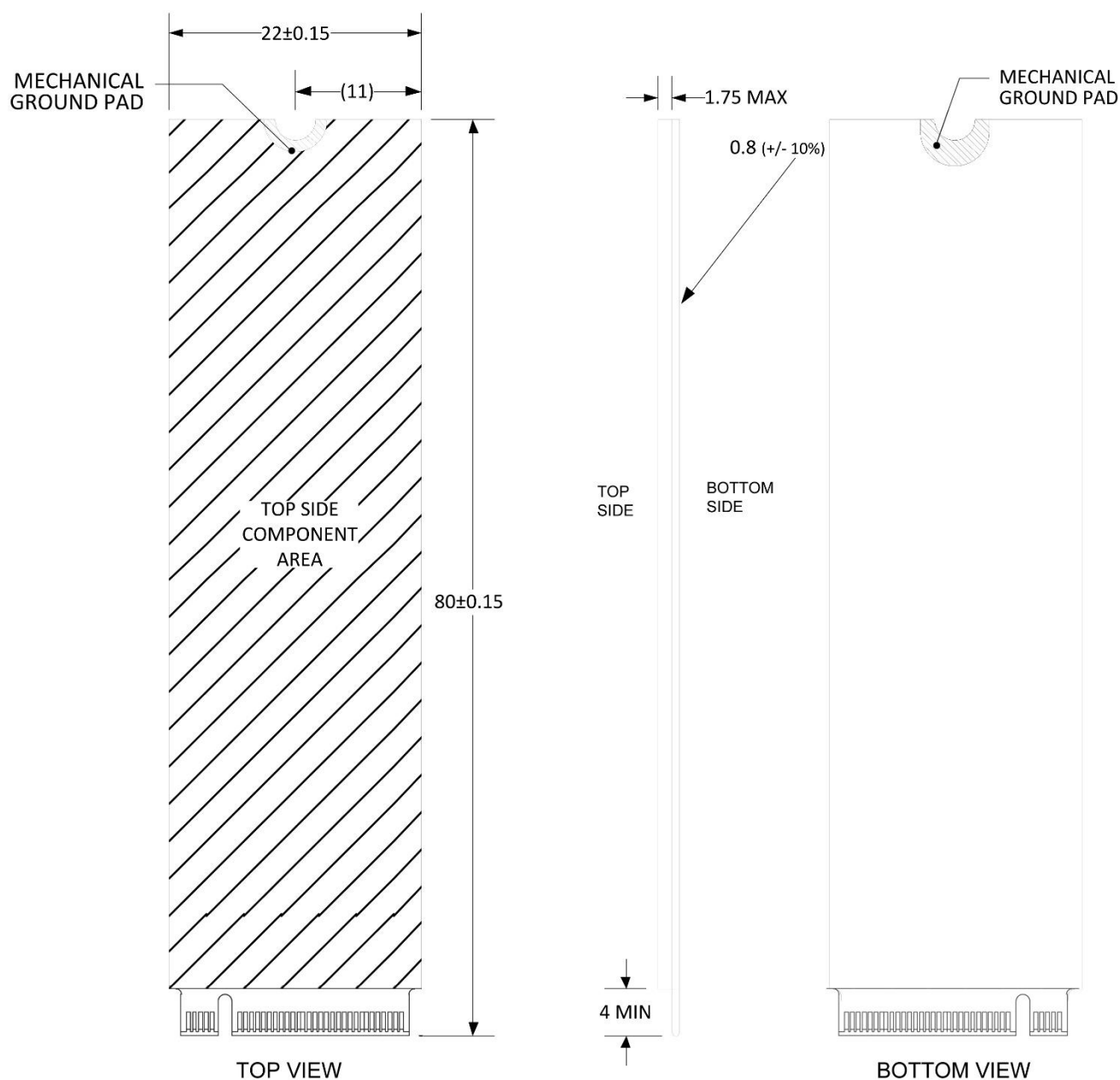
Figure 4: N3000 M.2 2280 dimensions in mm
