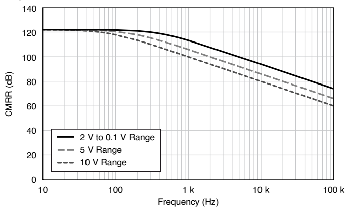
Figure 3. AI CMRR
