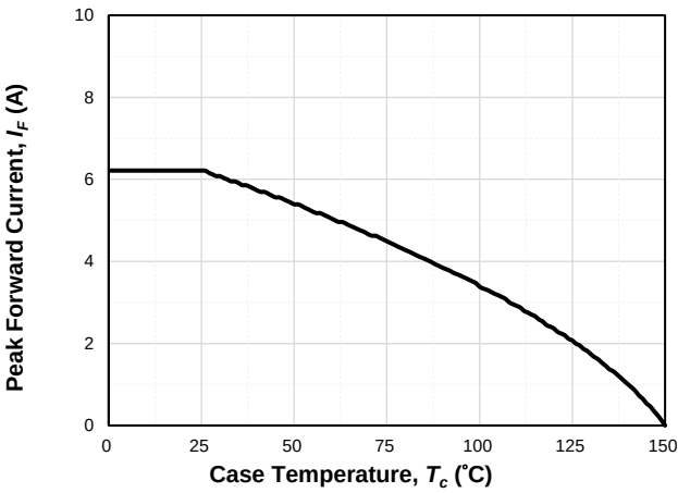
Fig. 8 Continuous I_F De-rating
