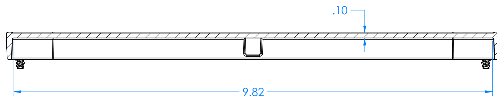
SECTION B-B
