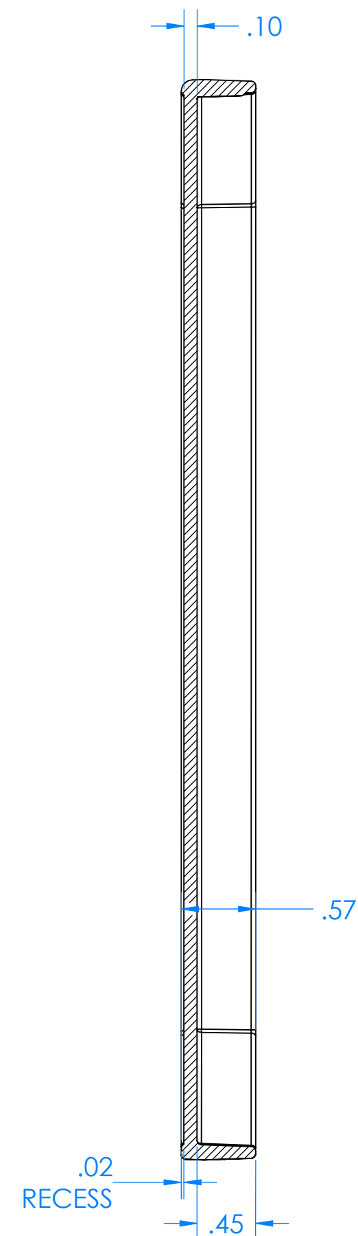
SECTION E-E
