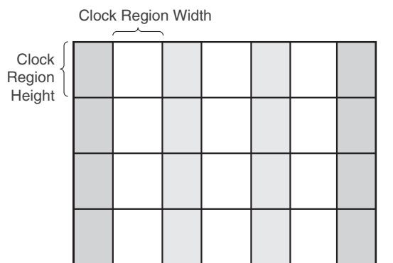
Figure 2: Column-Based FPGA Divided into Clock Regions
