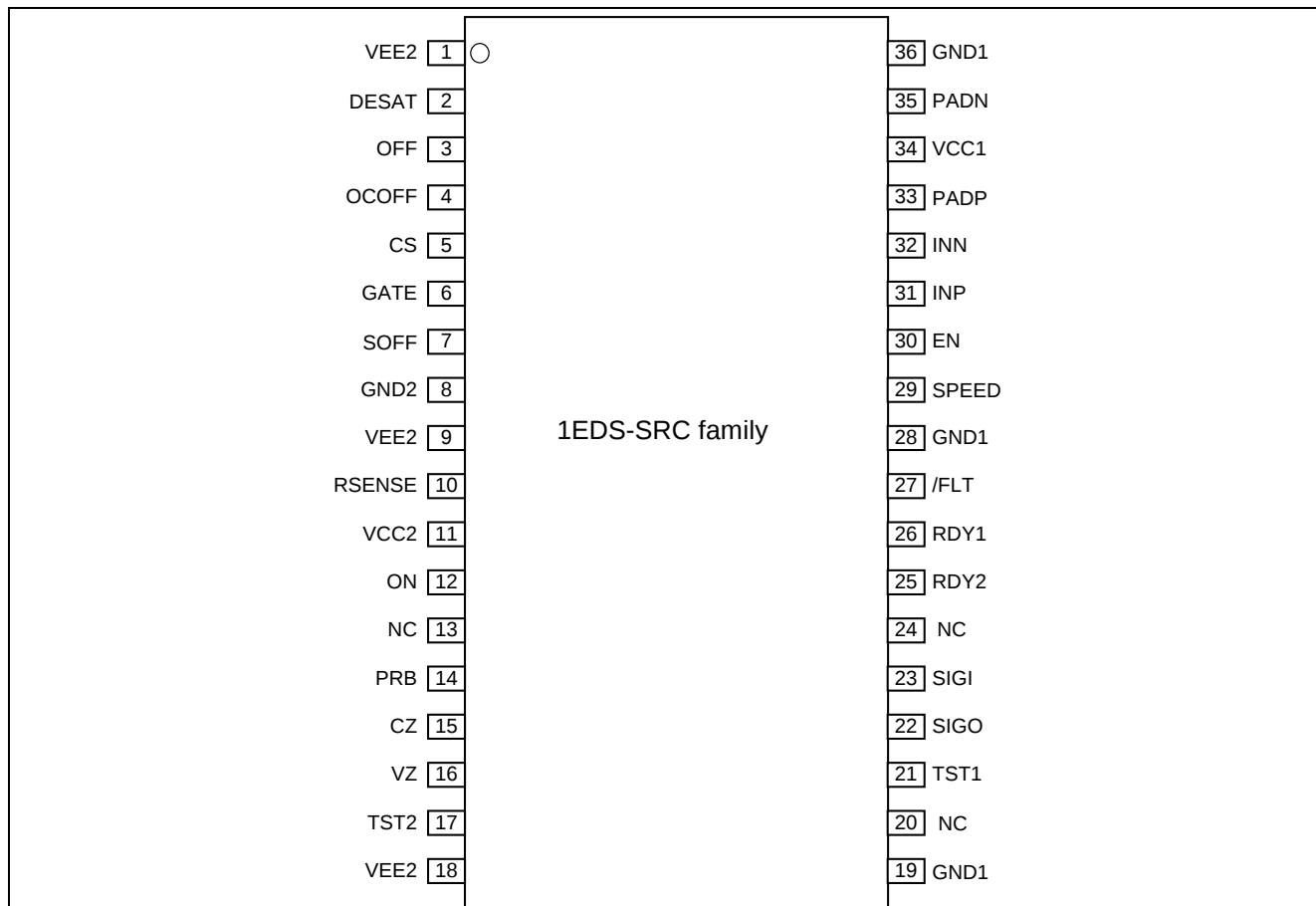
Figure 2 Terminal configuration of the 1EDS-SRC family (Top View)
