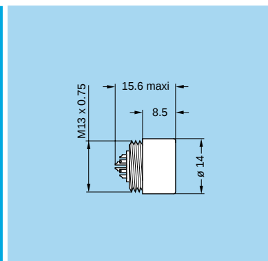
EYG.2G Fixed socket, key (G), protruding shell (screw fixing on the panel)
