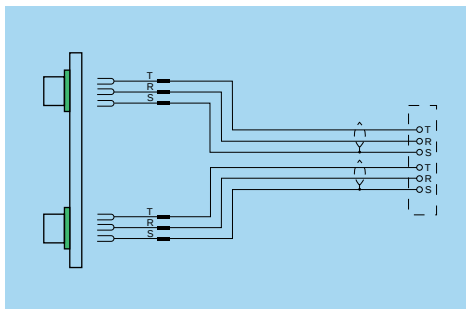
Rear side connection
