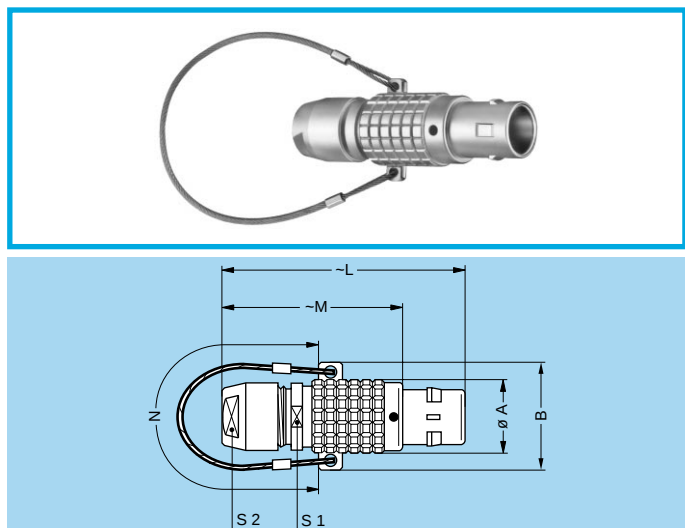
FNG Straight plug, key (G) or keys (A...M and R), cable collet and lanyard release
