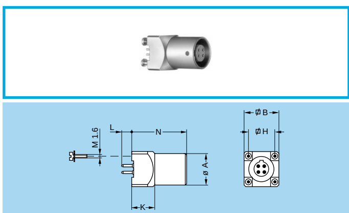
EZG Straight socket for printed circuit, key (G) or keys (A...F)
