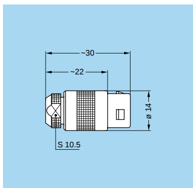
FGG.2G Straight plug, key (G), cable collet
