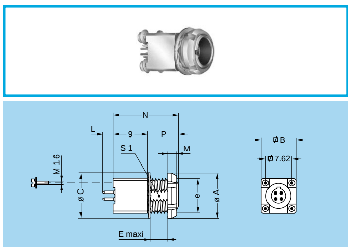
EYG Fixed socket for printed circuit, nut fixing, key (G) or keys (A...F) (back panel mounting)
