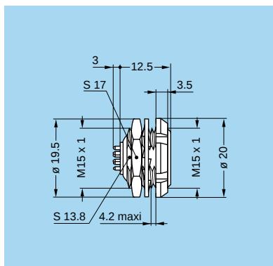
ECG.2G Fixed socket with two nuts, key (G), straight contact for printed circuit (back panel mounting)
