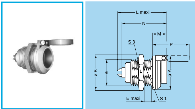
EVG Fixed socket, nut fixing, key (G) or keys (A to F and L) and dust cap (spring loaded)
