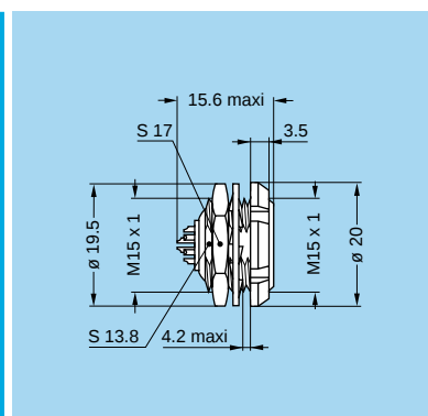
ECG.2G Fixed socket with two nuts, key (G) (back panel mounting)
