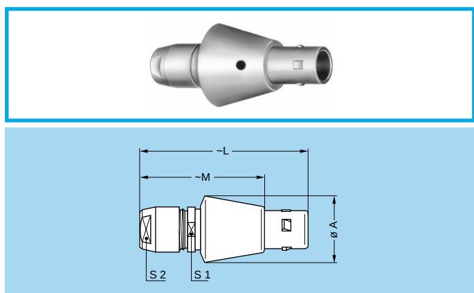
FYG Straight plug, conical shell, key (G) or keys (A...M), cable collet
