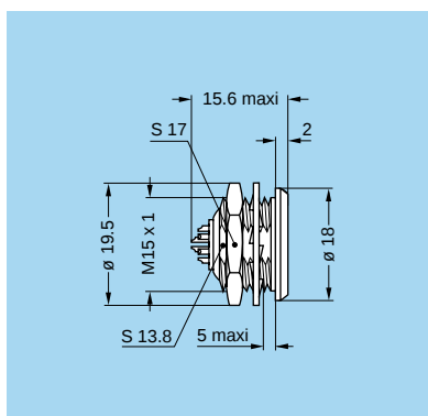
EGG.2G Fixed socket, nut fixing, key (G)
