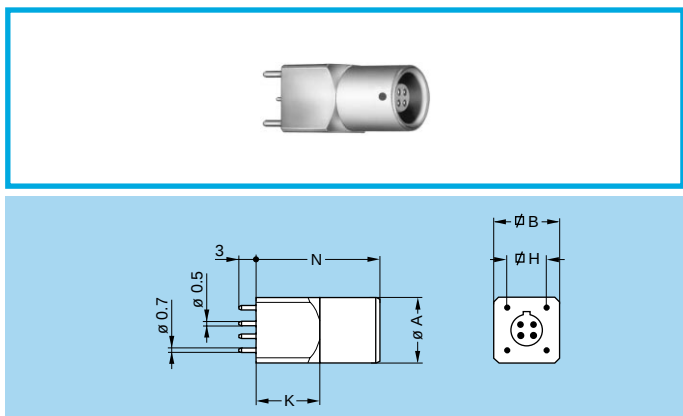
EZG Straight socket for printed circuit, key (G) or keys (A, B)
