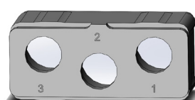
Insert Name 3T3 (1) Insert Code Z 3 x size 8 BMA pin contacts
