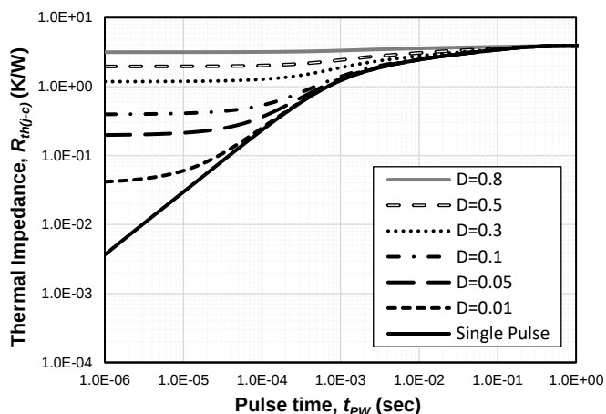
Fig. 8 Typ. Transient Thermal Impedance R_{th-jc} (TO-220FP-2L)
