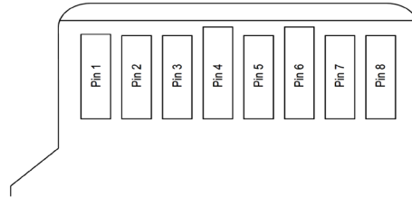
microSD Card Pin assignment (Back View of the card)
