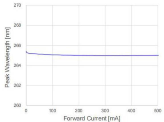
Forward Current vs. Peak Wavelength
