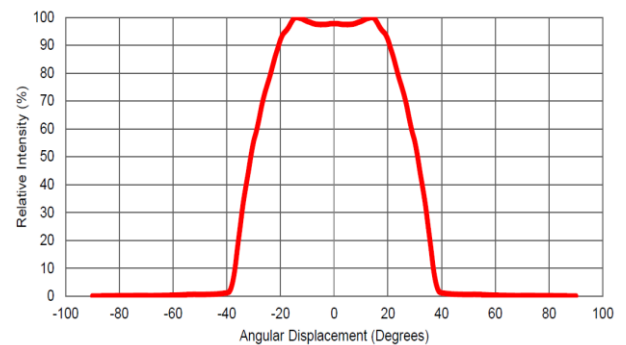
Radiation Pattern for 60 degree
