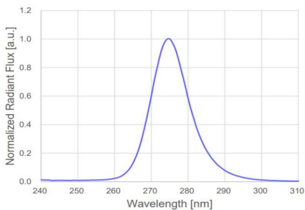
Spectrum Distribution
