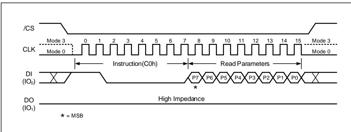
Figure 54a. Set Read Parameters Instruction (SPI Mode) "Set Read Parameters" command (C0h) can set the number of dummy clocks.
