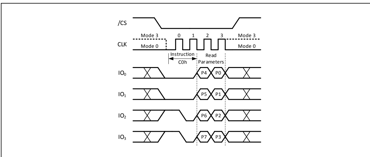
Figure 54b. Set Read Parameters Instruction (QPI Mode) "Set Read Parameters" command (C0h) can set the number of dummy clocks.
