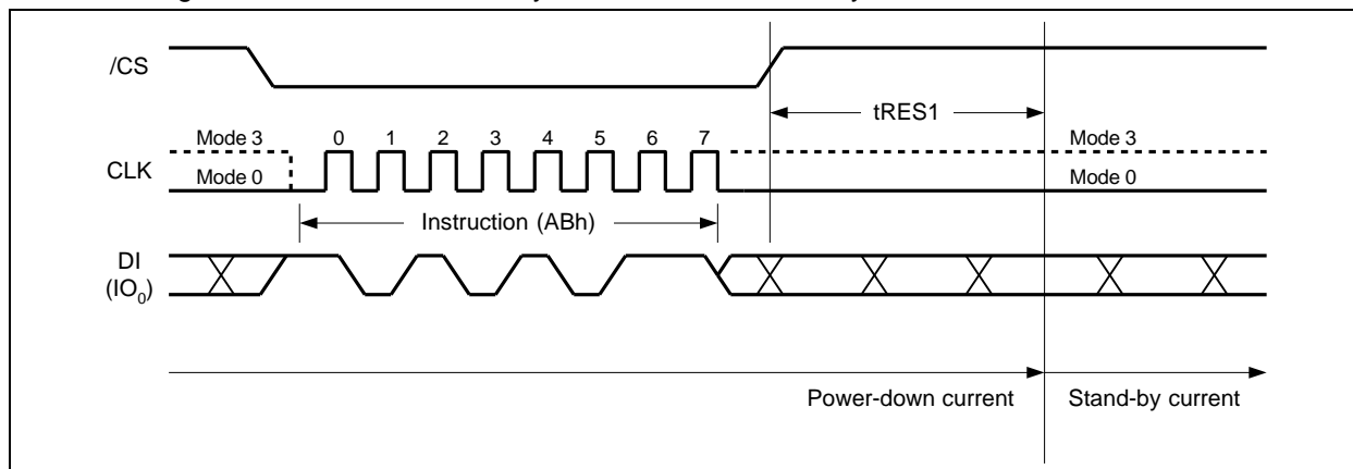
Figure 38a. Release Power-down Command (SPI Mode)
