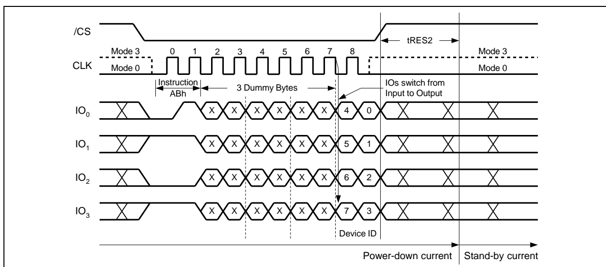
Figure 38d. Release Power-down / Device ID Command (QPI Mode)
