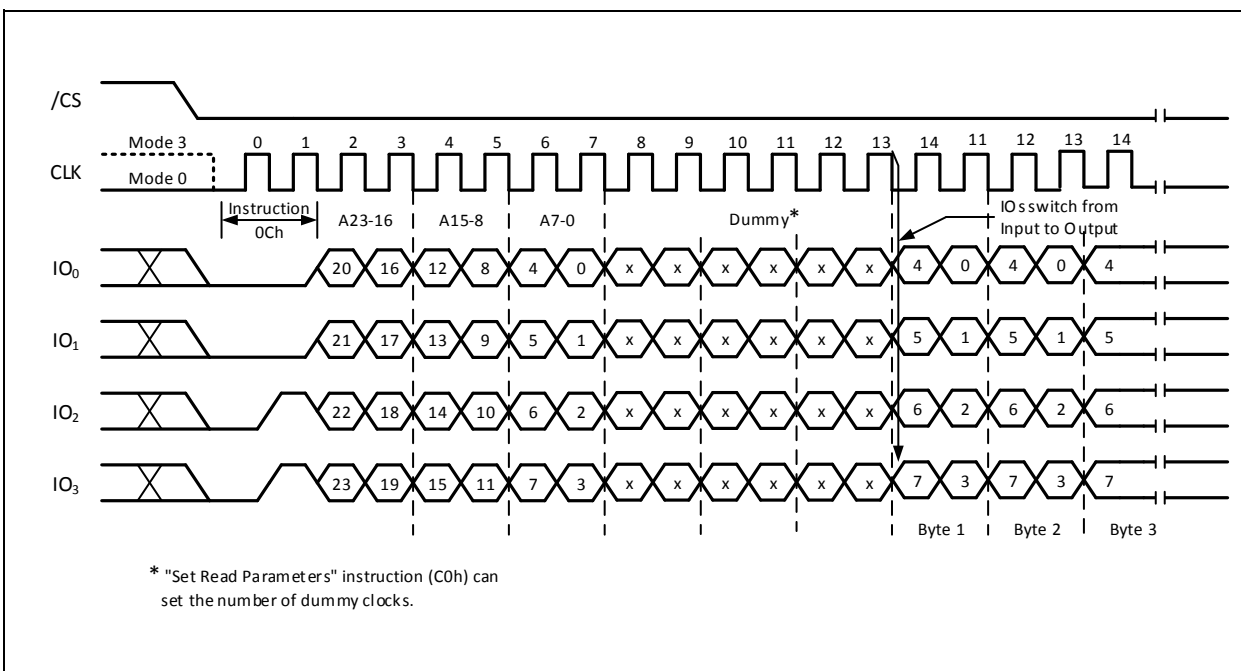
Figure 48. Burst Read with Wrap Command (QPI Mode only)
