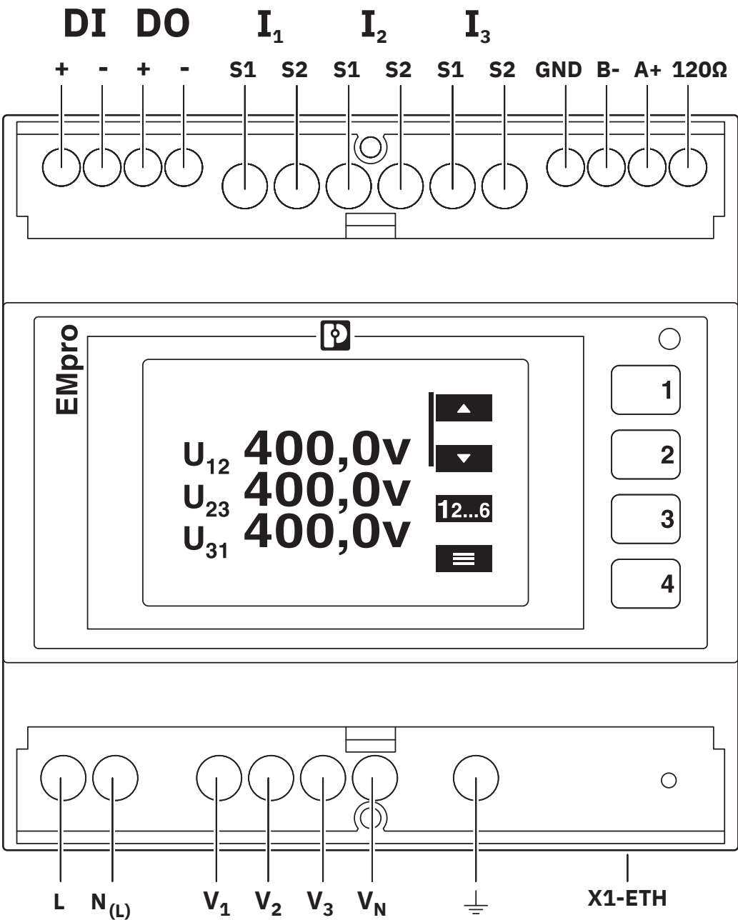
Connection diagram
