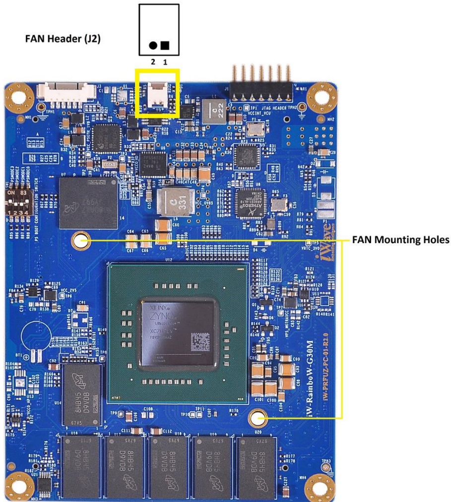
Figure 6: Fan Header
