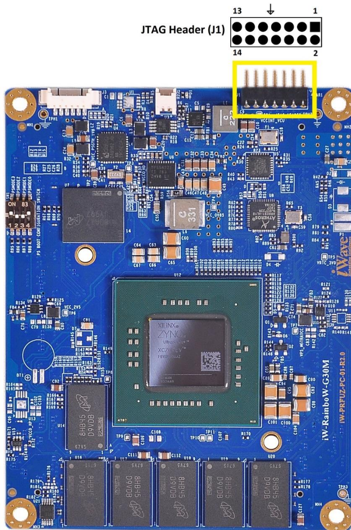
Figure 5: JTAG Header
