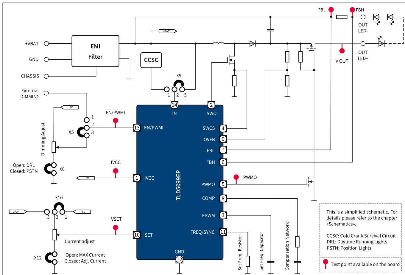
Figure 2 Simplified schematic
