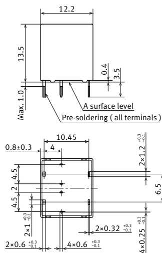
External dimensions
