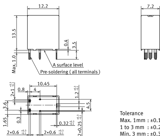
External dimensions
