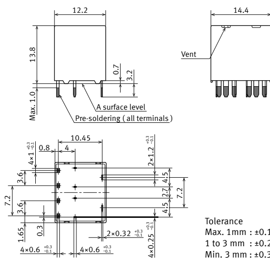
External dimensions
