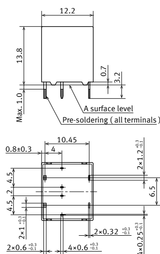
External dimensions
