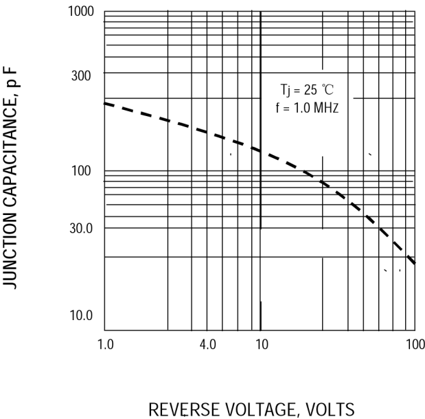
FIG.2-TYPICAL JUNCTION CHARACTERISTICS
