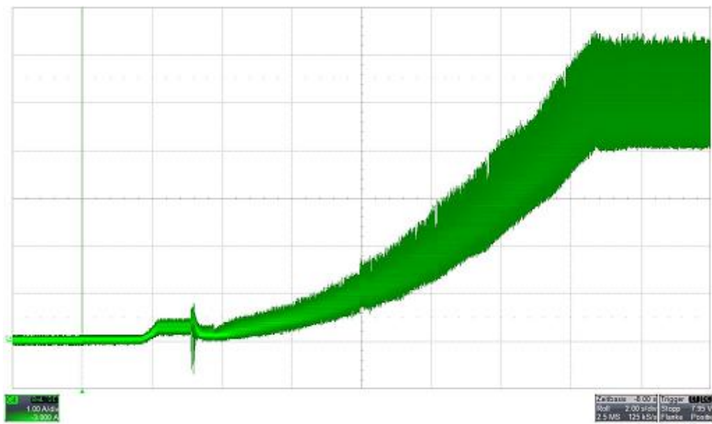
Startup current @ 24V, 0 - 11000 rpm
