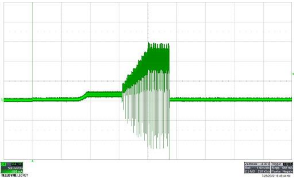
Locked rotor current @ 30V
