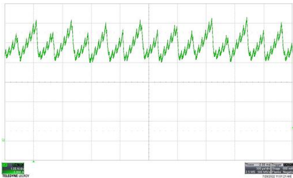
Running current @ 24V, free blowing, 11000 rpm
