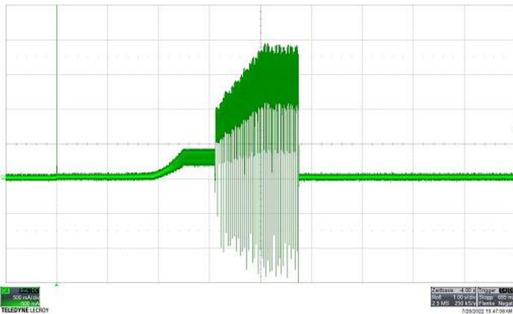
Locked rotor current @ 16V
