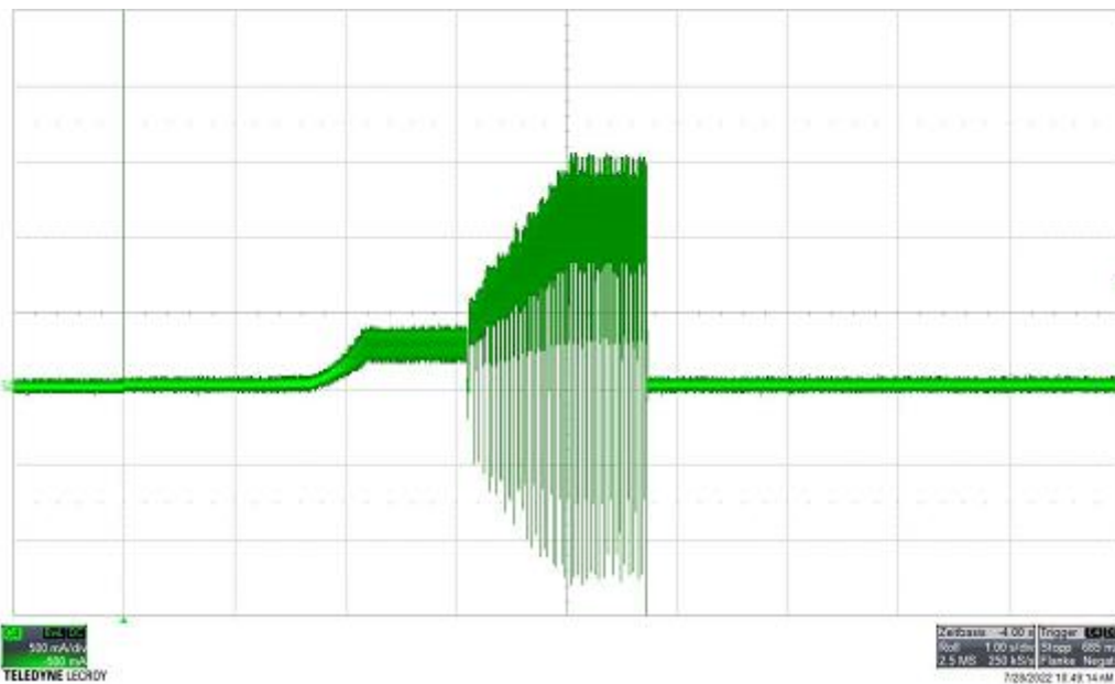
Locked rotor current @ 24V
