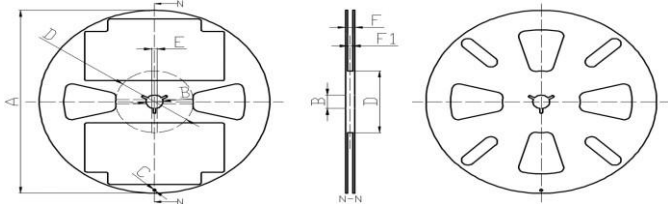
Fig. 6-2 Disc (Width of carrier-16 mm)
