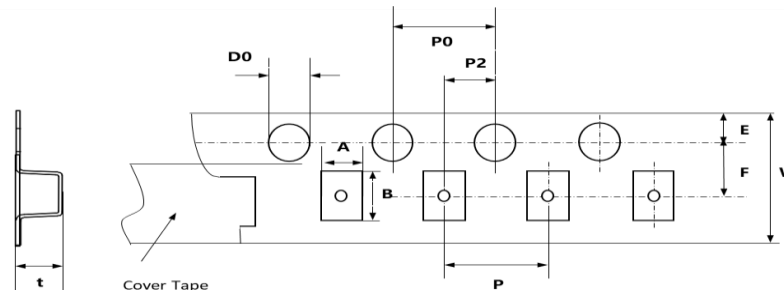
Fig. 5-2 0603, 0805, 1206, 1210 (Plastic tape)
