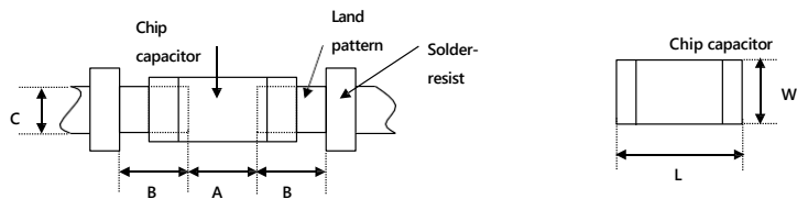
Recommended land dimensions for reflow-soldering
