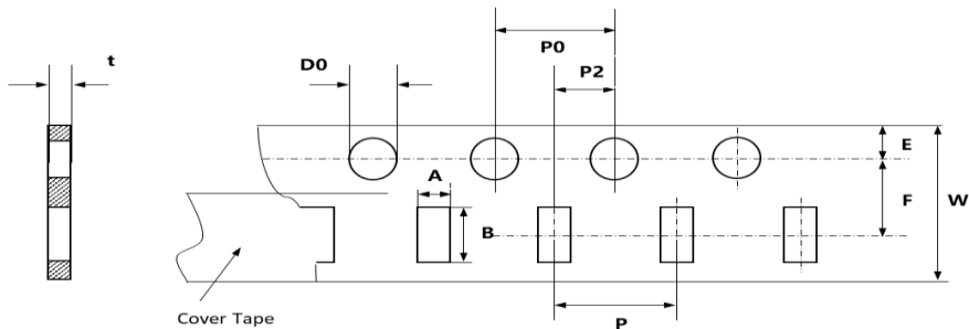
Fig. 5-1 0603, 0805, 1206, 1210 (Paper tape)
