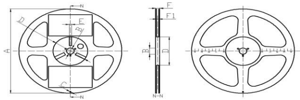
Fig. 6-1 Disc (Width of carrier-8 mm)
