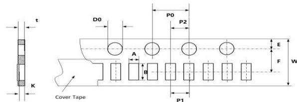
Fig. 7-2 0201 (Paper tape/ 2 mm pitch)
