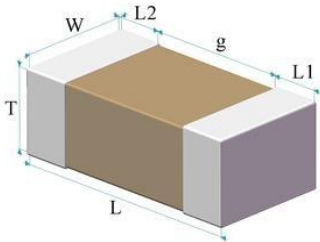
Fig.1 Structure & Dimension
