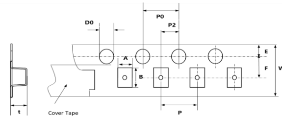
Fig. 7-5 0603,0805,1206,1210 ,2220 (Plastic tape)
