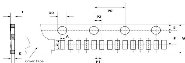
Fig. 7-3 0201 (Paper tape/ 1 mm pitch)
