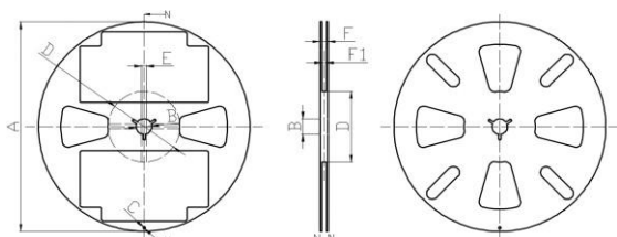
Fig. 8-2 Disc (Width of carrier-16 mm)
