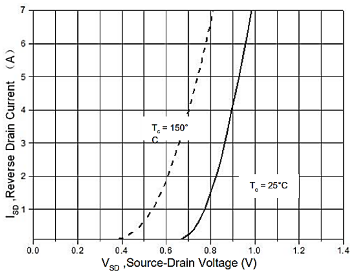
Figure 12. Body Diode Transfer Characteristics
