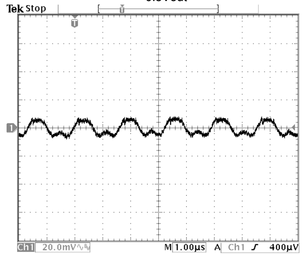
Fig.11: Output ripple and noise at 5.0Vin, 3.465V/6Aout
