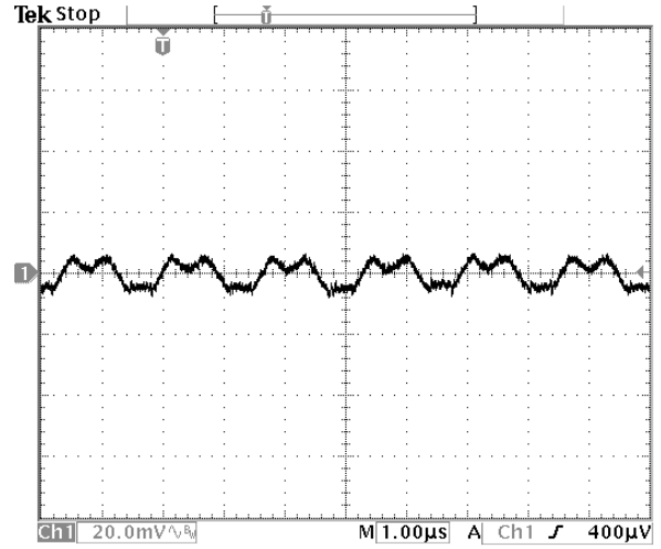
Fig.15: Output ripple and noise at 5.0V in , 0.8V/6Aout
