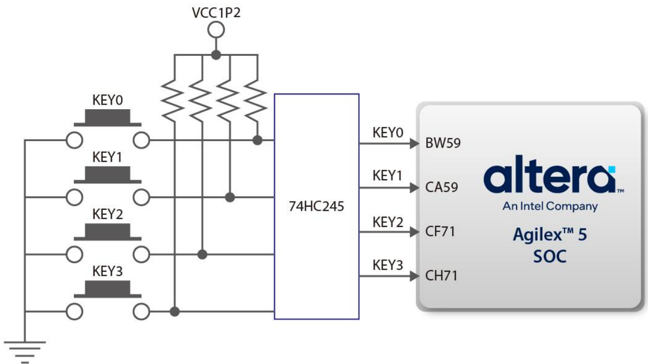
Figure 3-18 Connections between the push-buttons and the Agilex 5 SoC FPGA
