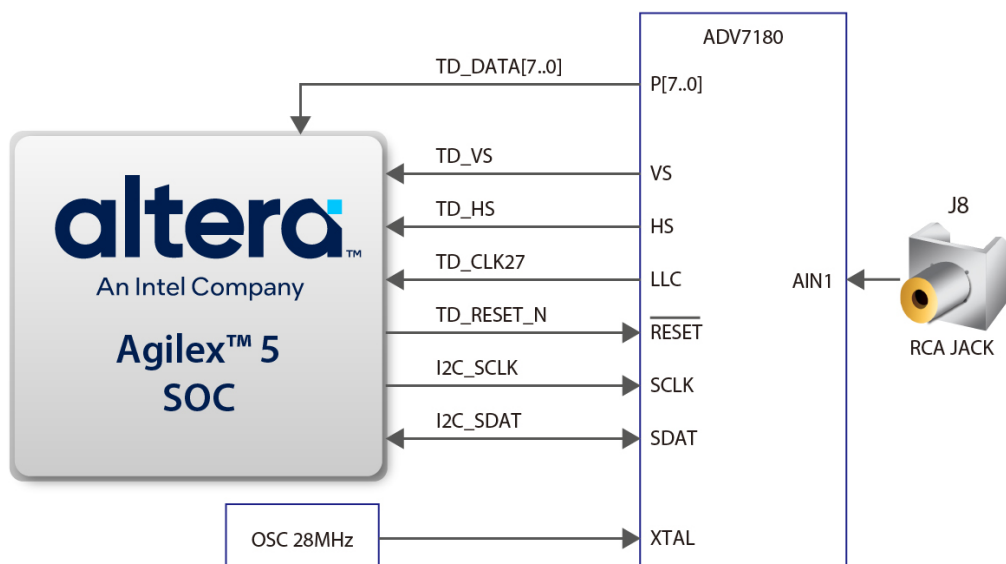
Figure 3-27 Connections between the FPGA and TV Decoder
