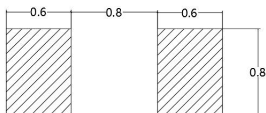
建议焊盘尺寸 Recommended Soldering Pattern
