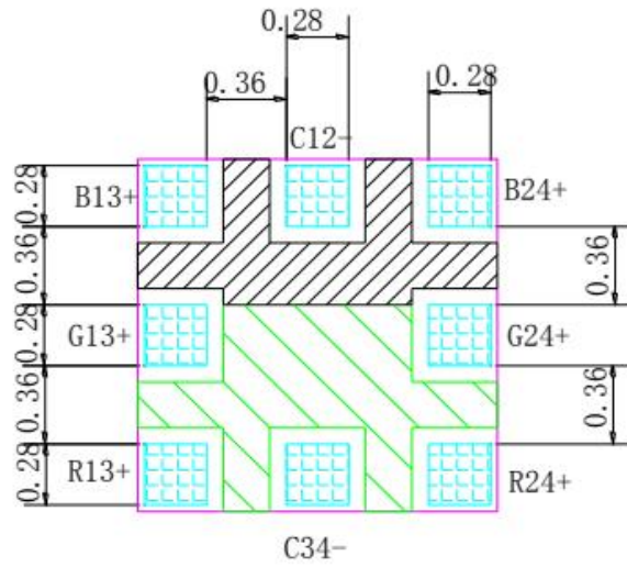
建议焊盘尺寸: Recommended Soldering Pattern
